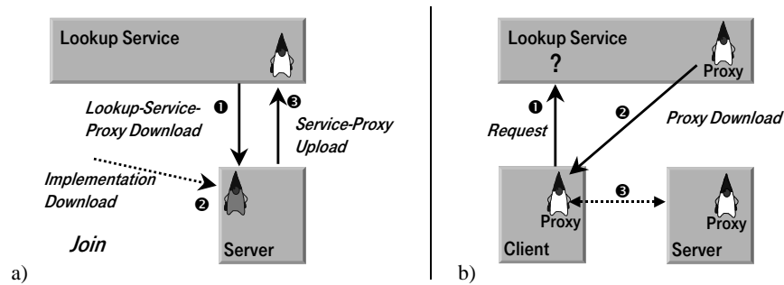
Fig. 1. Jini-Protocols: a) Discovery/Join and b) Lookup
